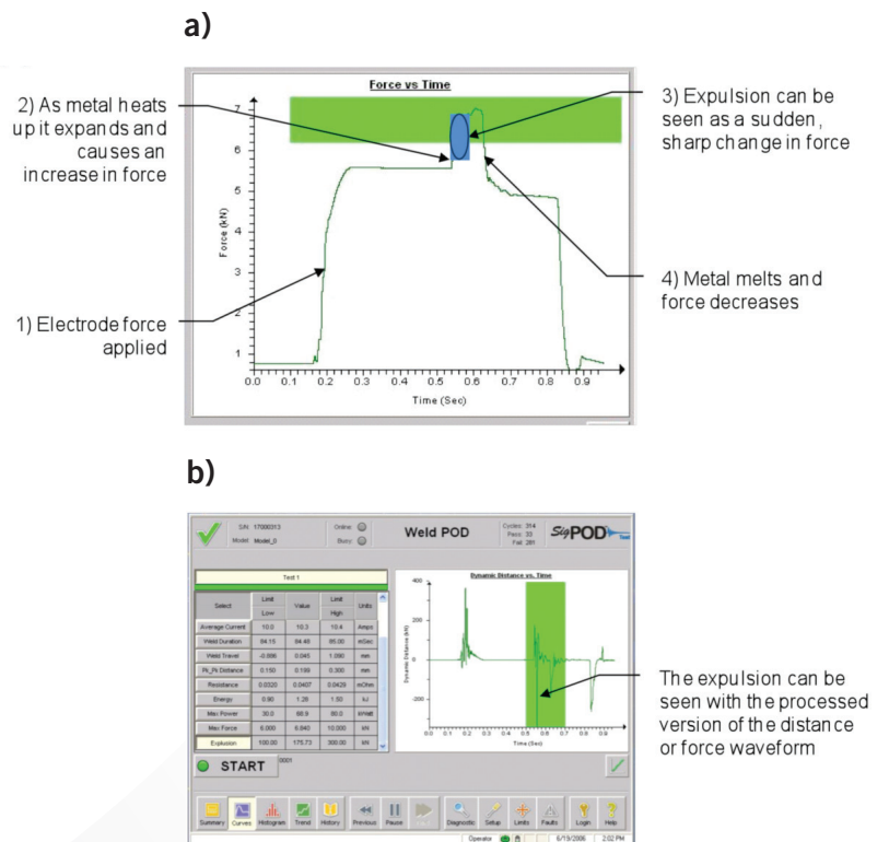
Figure 5: Force vs. time weld signature showing evidence of an expulsion event. Detection of these rapid changes in force can be enhanced by looking at the derivative of the force vs. time signature, as illustrated in (b).
